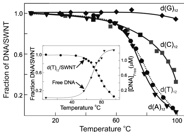
Figure 2. Nucleobase dependence of DNA/SWNT dissociation. The fraction of total initial DNA/SWNTs that remained suspended after 10 min. was plotted as a function of temperature for poly d(G) 12 , d(C) 12 , d(T) 12 , and d(A) 12 and fitted to the sigmoidal function y = y_0 + a/(1 + e^{-b(T - T_{1/2})}) , where T is the temperature in degrees Celsius and a , b and y_0 are parameters of the fit. Inset: results of an independent experiment with nanotubes associated with dT 12 DNA in which the measured concentration of free DNA unbound from the d(T) 12 /SWNTs after 10 min as a function of temperature was superimposed on the plot showing the fraction of d(T) 12 /SWNT that remained suspended.
