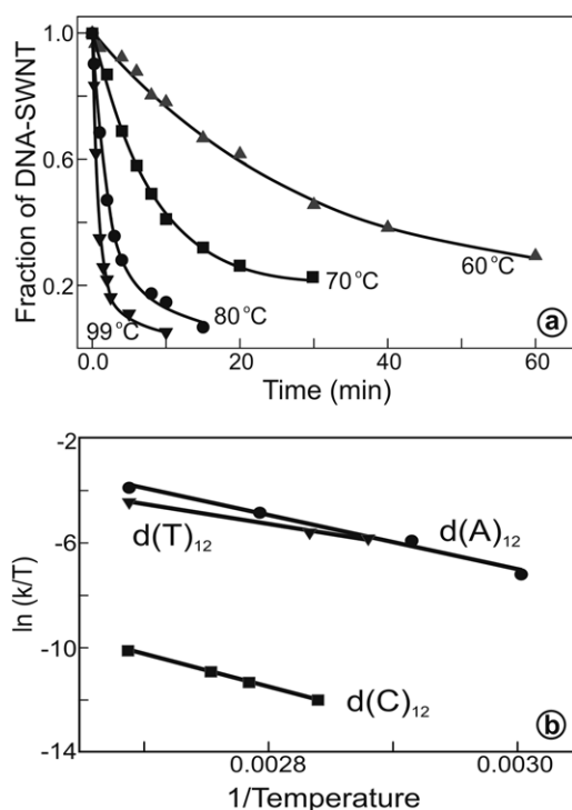
Figure 6. Temperature dependence on the rate of hybrid dissociation. (a) The fraction of total initial d(A) 12 /SWNTs that remained suspended plotted as a function of time at four different temperatures. (b) Eyring plots of similar data for nanotubes associated with poly d(A) 12 , d(C) 12 , and d(T) 12 . The slopes of the lines reveal the activation enthalpy of DNA unbinding from nanotubes (table 1) and show the same nucleobase trend as observed in the isochronal temperature plots of figure 2.
