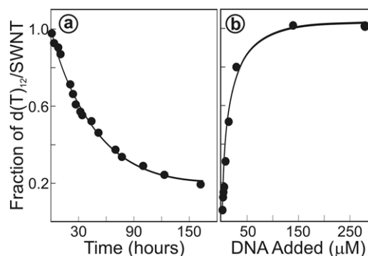
Figure 4. Dissociation kinetics of d(T) 12 /SWNT at room temperature. (a) The solid line is a fit to an exponential decay with a fractional offset d = 0.22 (see equation (2)) and a T_{1/2} for the first order process (41 h). (b) The fraction of total initial dispersed d(T) 12 /SWNTs that remained suspended after 480 h at room temperature as a function of free DNA added at t = 0 h.
