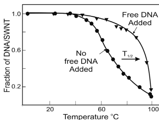
Figure 5. Tuning the thermal dissociation of DNA/SWNTs. Upon addition of 140 \mu\text{M} free poly d(T) 12 ssDNA to a d(T) 12 /SWNT dispersion, the hybrid dissociation temperature ( T_{1/2} ), measured by the isochronal temperature assay, was shifted to a higher temperature.
