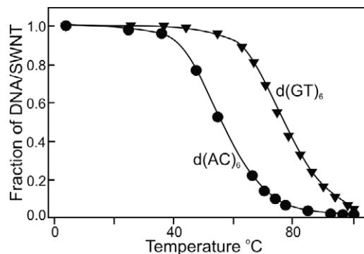
Figure 3. Effect of alternating bases on DNA/SWNT stability. The fraction of total initial DNA/SWNTs that remained suspended after 10 min was plotted as a function of temperature for poly d(AC) 6 /SWNTs and d(GT) 6 /SWNTs.
